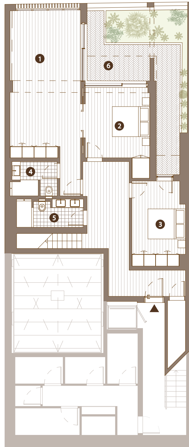
Piso -1 Floor -1
